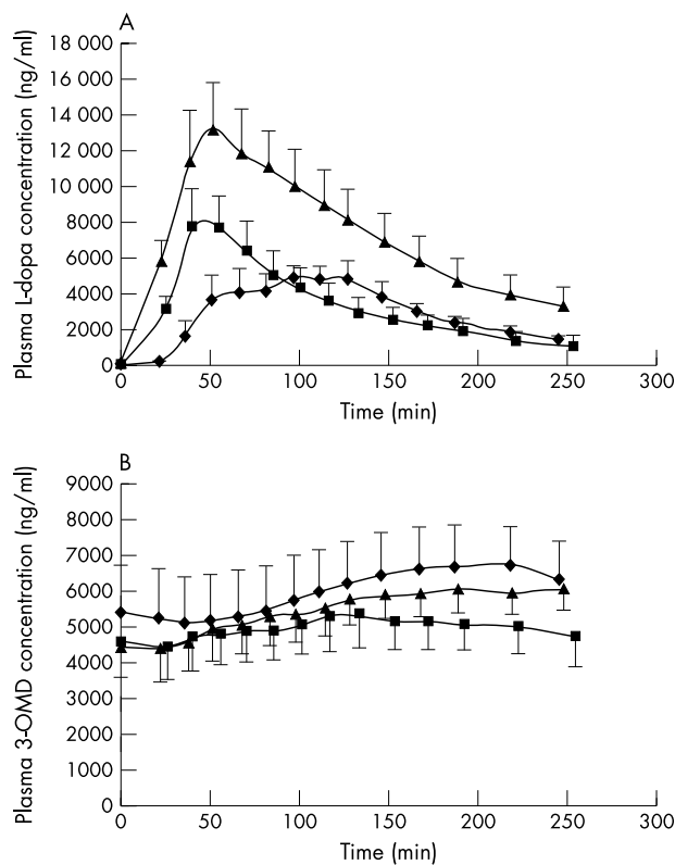
Figure 1 (A) Plasma concentration v time profiles for L-dopa following ingestion of 200 mg L-dopa/50 mg carbidopa (◆), 15 g mucuna (■), or 30 g mucuna (▲) seed powder. Data are mean (SEM) of eight patients. (B) Plasma concentration v time profiles for 3-OMD following ingestion of 200 mg L-dopa/50 mg carbidopa (◆), 15 g mucuna (■), or 30 g mucuna (▲) seed powder. Data are mean (SEM) of eight patients.
